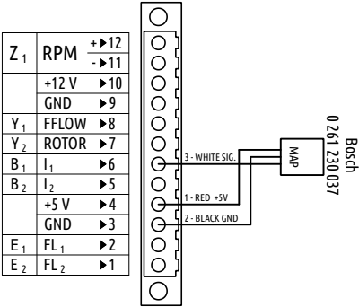
Figure 35: External MAP sensor from Bosch, connection schematics.
