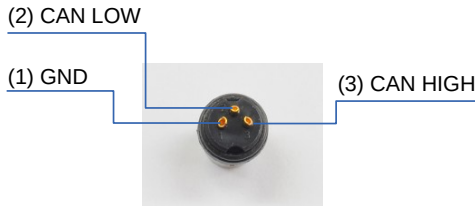
Figure 38: Photo of connector back side. Note the three small numbers, which define the pin positions. GND is usually not connected.
