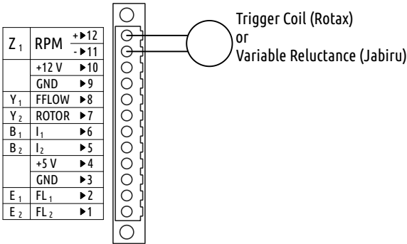
Figure 31: Connection of trigger coil sensor or variable reluctance sensor to Z channel.
