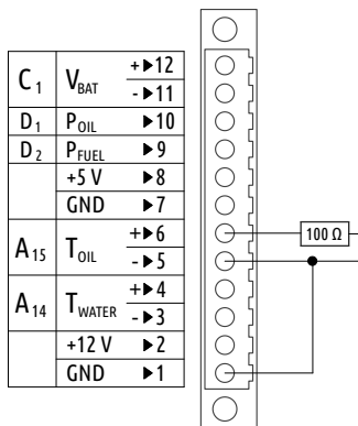
Figure 42: Example: VDO oil temperature sensor was replaced by a known test resistor. A 100 \Omega resistor is shown, but any other test resistor from Table 35 can be also used.
