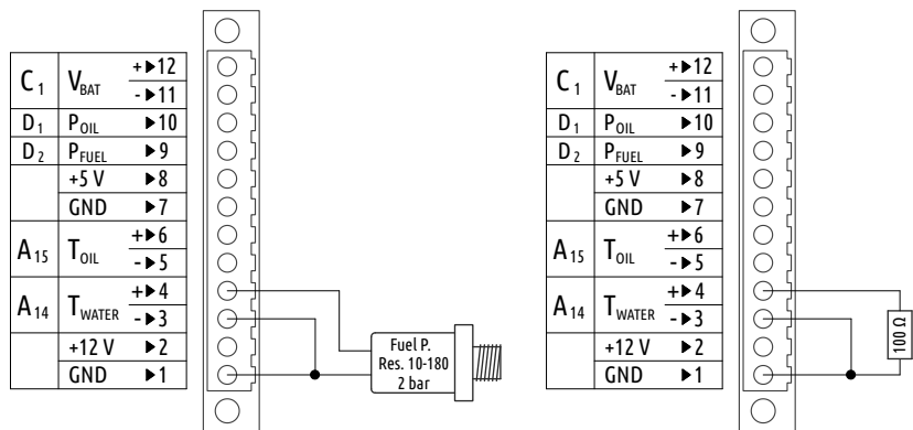
Figure 40: Example: VDO 2 bar sensor was replaced by a fixed 100 Ohm resistor.
