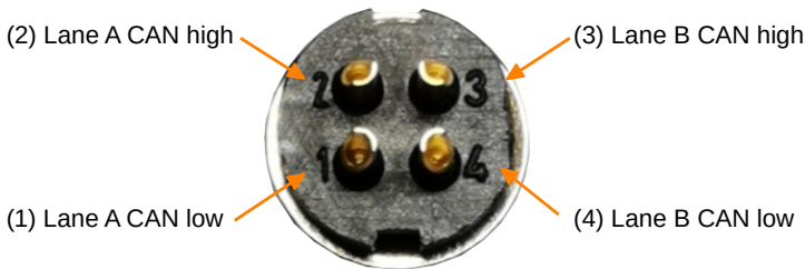
Figure 39: Cable plug back side. Note the four small numbers, which define the pin positions inside the plug. This is Binder part number 99 0979 100 04.
