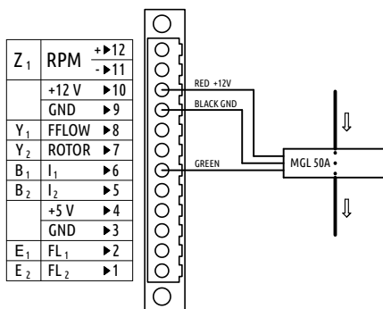
Figure 28: MGL 50A Close Loop sensor connection schematics.
