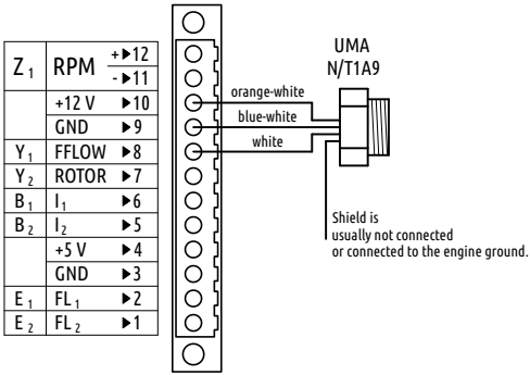
Figure 32: Connection of UMA T1A9 or N1A9 sensor to Y channel. Any Y channel can be used.
