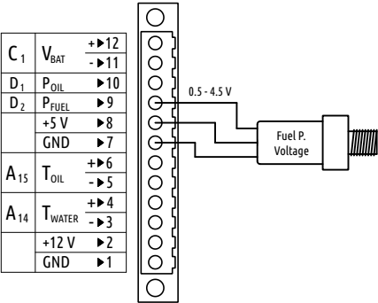
Figure 23: Fuel pressure sensor with variable voltage (0.5 – 4.5 V) output. Sensor is powered with 5V.
