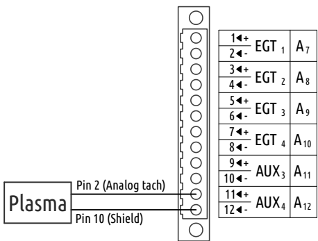
Figure 33: Connection of Plasma RPM analogue voltage output signal to A channel.
