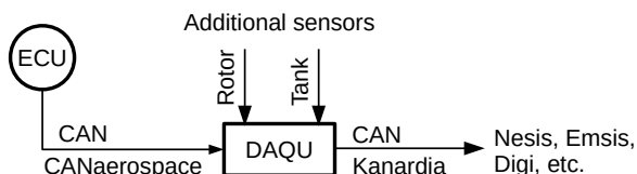
Figure 36: Illustration of the connection principle. Almost all information comes from the ECU. Rotor RPM and fuel tanks and other additional sensors can be still connected directly to Daqu.
