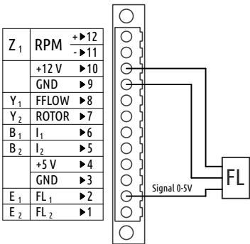
Figure 30: An example of capacitive fuel level probe connected to the +12 V power source. Some probes require 5 V, be careful.
