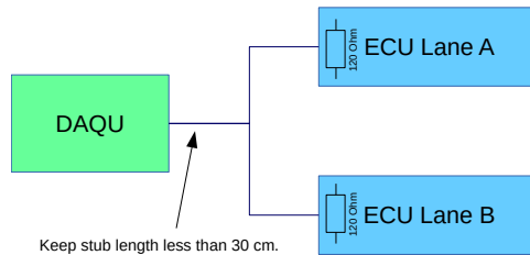
Figure 37: CAN bus connectivity.
