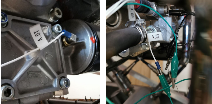
Figure 41: Test setup. Left: Location of the oil temperature sensor and its lead to Daqu (labeled as A.OT). Right: Oil temperature lead was detached and connected with green cable to one side of the test resistor. The other side of the resistor connects to an appropriate engine point (black cable).
