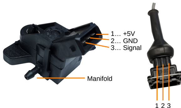
Figure 34: External manifold pressure sensor, Bosch 0 261 230 037.
