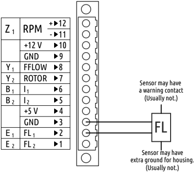
Figure 29: An example of resistive fuel sensor. Usually it has only two connections. But it can have more. Please refer to the sensor manual for more details.
